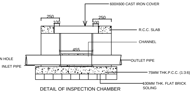
DETAIL OF INSPECTION CHAMBER
