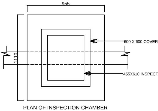
PLAN OF INSPECTION CHAMBER
