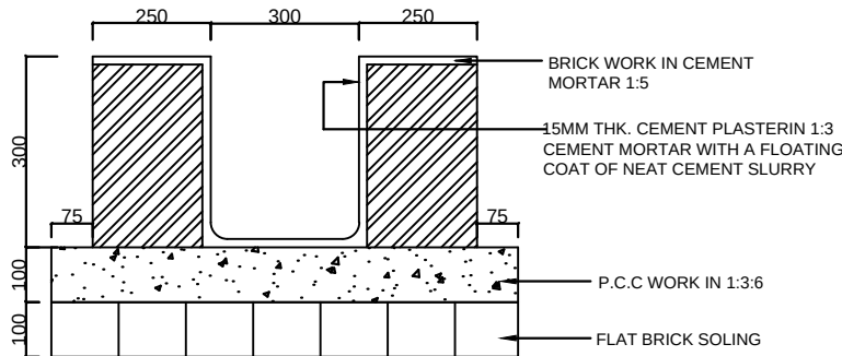
TYPICAL DETAIL OF HOUSE DRAIN
